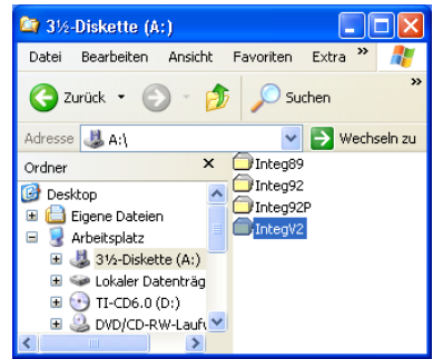
Abb. 1.4 Windows Explorer
